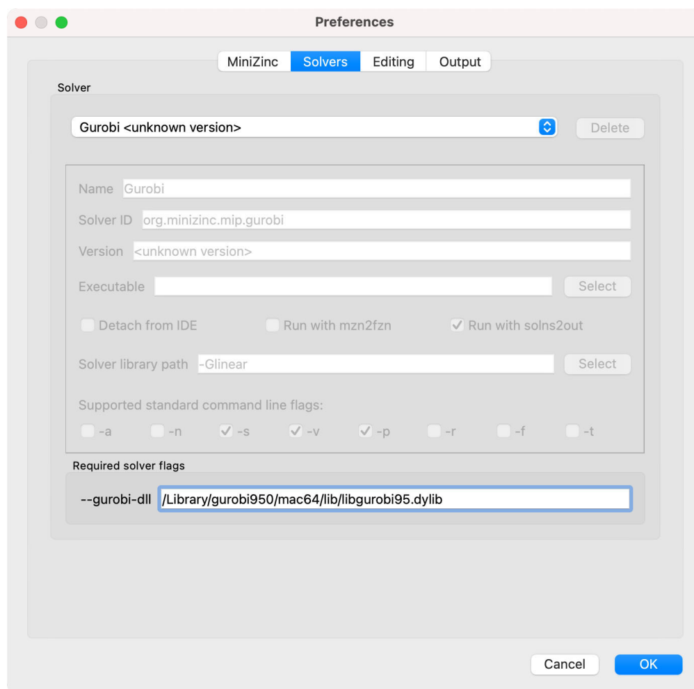
图 2.7: Configuring the Gurobi DLL path
