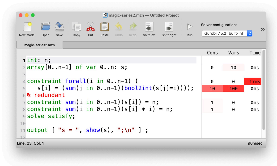
图 2.2: Profiling results for the Magic Series problem ( n=10 )
