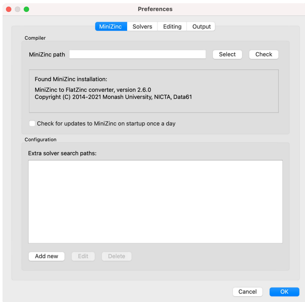
图 2.5: The MiniZincIDE preferences window
